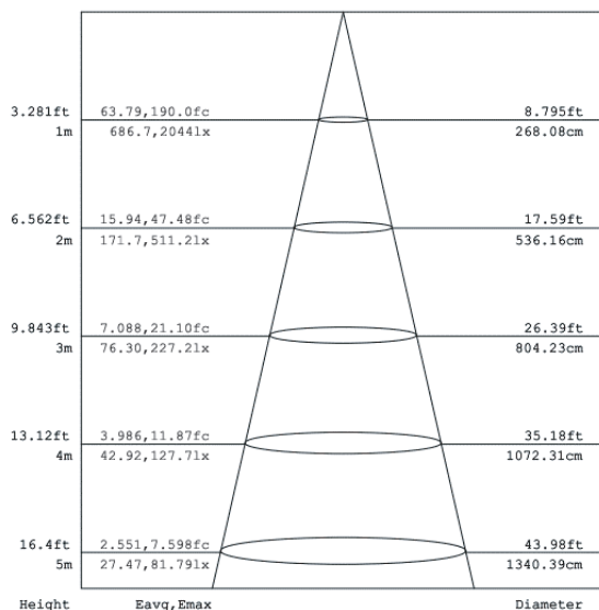
Cone illuminance Diagram:
